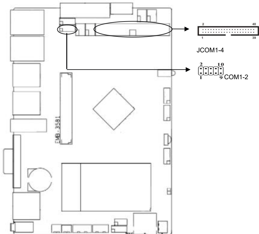
COM1-2: 2*5PIN 2.00MM 排针
